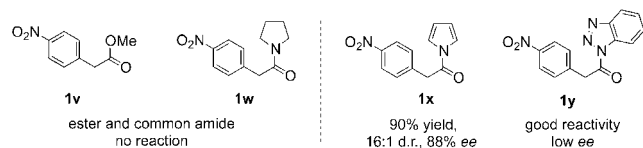
Scheme 4. Control experiments in support of the proposed mechanism.
